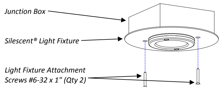
Figure 4 - Mounting Light Fixture to Junction Box
