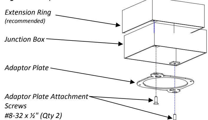
Figure 2 - Adaptor Plate Installation
