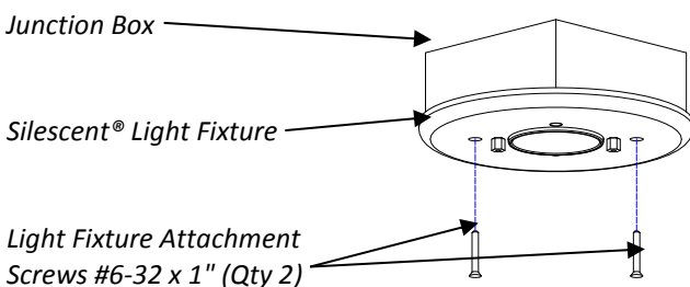
Figure 4 - Mounting Light Fixture to Junction Box
