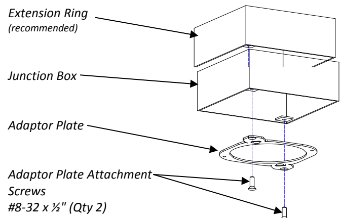
Figure 2 - Adaptor Plate Installation
